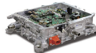
Integrated On-Board Charger and DC-DC Converter Unit
